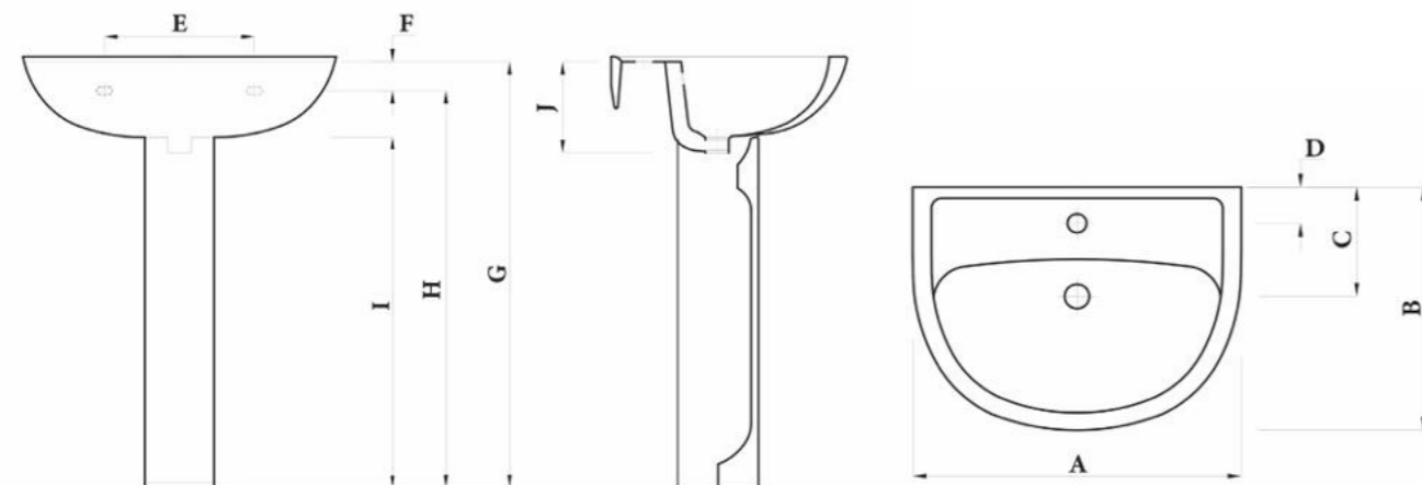
Shown : 63cm Basin & Pedestal. Available with 1 tap hole only with Milano mixer.
