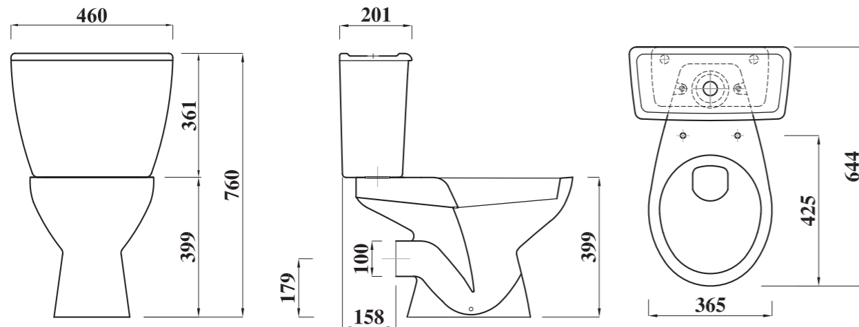
Shown :Close Coupled WC Suite, available in (P & S) trap. With douche, and push button flush.
