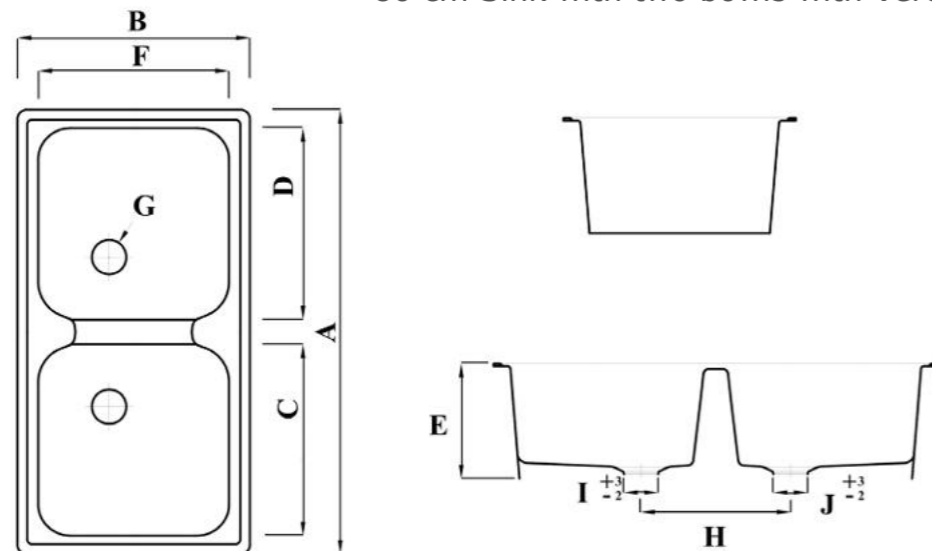
Shown : 80 cm Sink with two bowls with Verona mixer.
