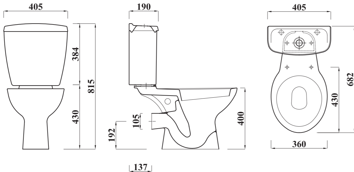
Shown : Close Coupled WC Suite, available in (P & S)trap. Available with douche and push bottom flush.
